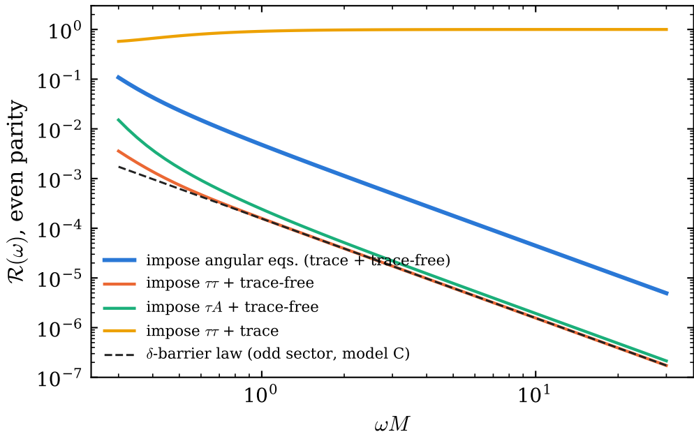
Frozen domain wall ( R = 6M , \ell = 2 ): the answer depends on a choice
